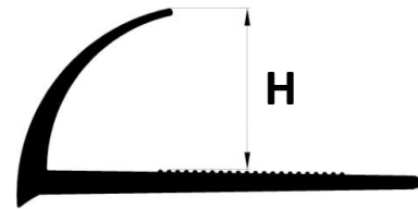
YJ-PPE H:10mm
