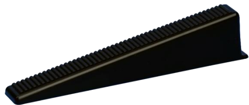
88X12X37mm
