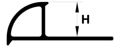
YJ-CT H:8/10/12/12.5mm
