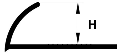
YJ-RT H:6/8/10/12/12.5mm
