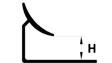
YJ-WT H:8/10/12mm
