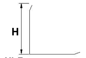
YJ-Z H:10/12/15/18/20/ 22/25/28/30/35/38 /40mm
