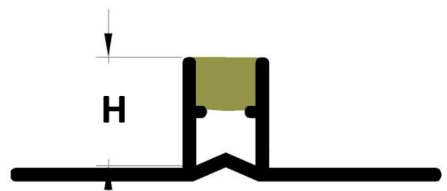
YJ-RT H:6/8/10/12/12.5mm
