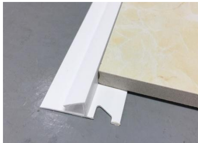
YJ-TV Height:12mm
